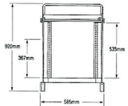
Figure 12. Keysight 1181BZ testmobile cart dimensions.
